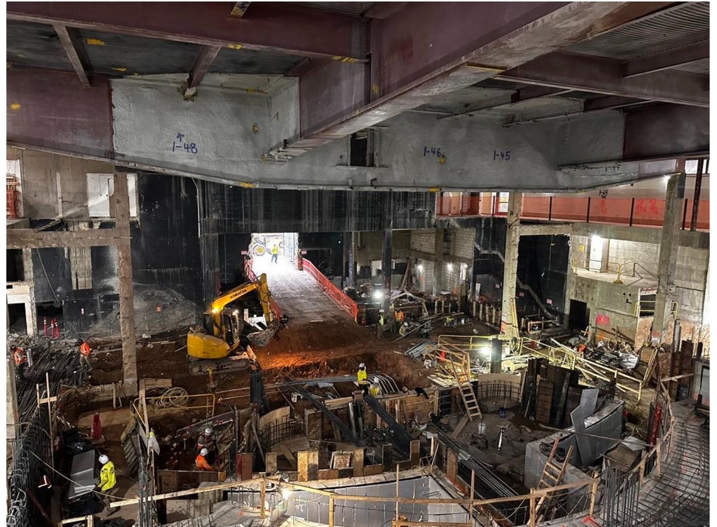
Continued rebar installation in the Large Venue in preparation for the concrete slab on grade.
