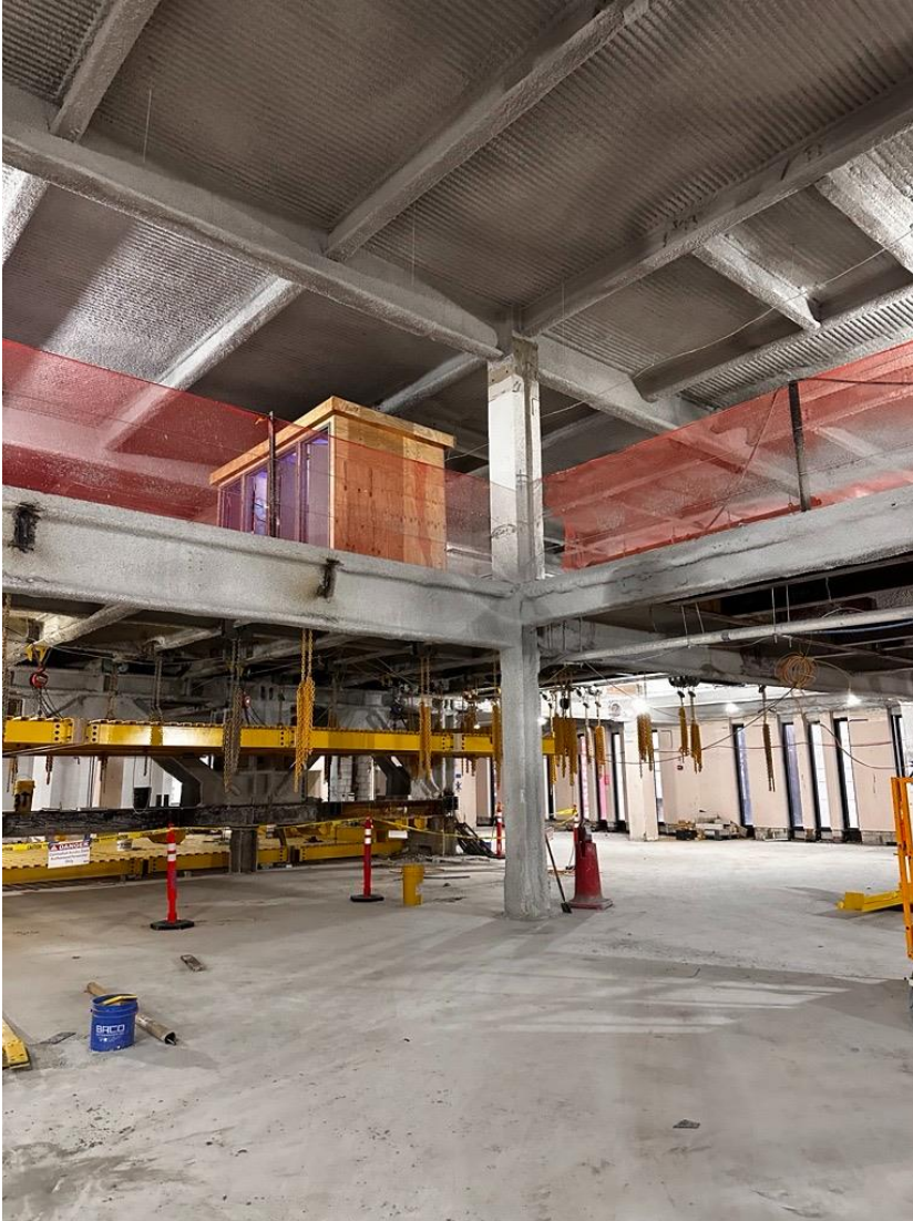
Grid iron being temporarily hung on the 2 nd floor.
